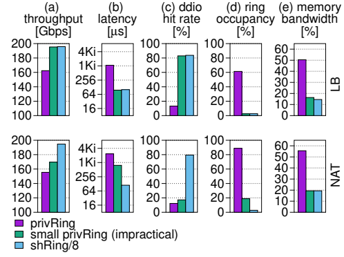
Figure 5.6: LB and NAT performance at 200Gbps load.
