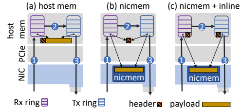
Figure 2.4: Host memory based packet transmission compared to data on nicmem with and without header inlining.
