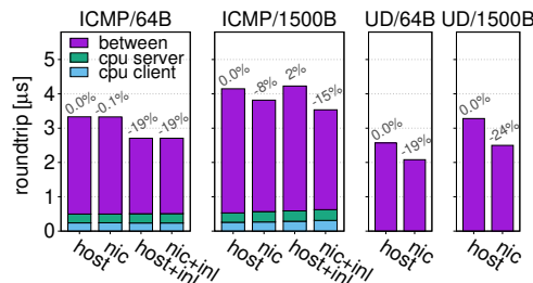
Figure 2.1: Superfluous data movement between NIC and host memory degrades performance even in underloaded conditions.
